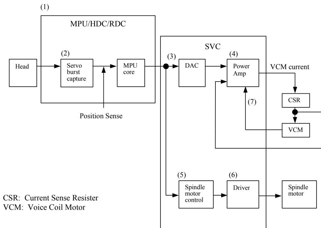
Figure 4.6 Block diagram of servo control circuit
